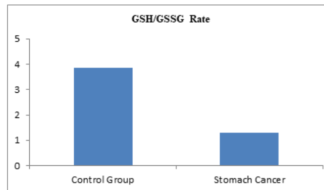
Figure 4: GSH/GSSG values
