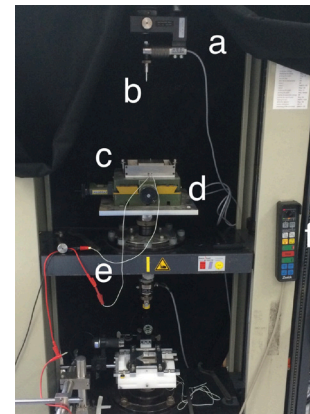
Fig. 3. Punch adapter machine
