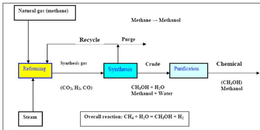
Figure 2. Schematic diagram shows methanol production (Omer, 2006).
