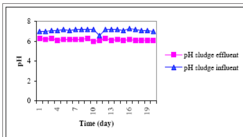
Figure 6. pH sludge before and after treatment in the digester (Omer, 2006).
