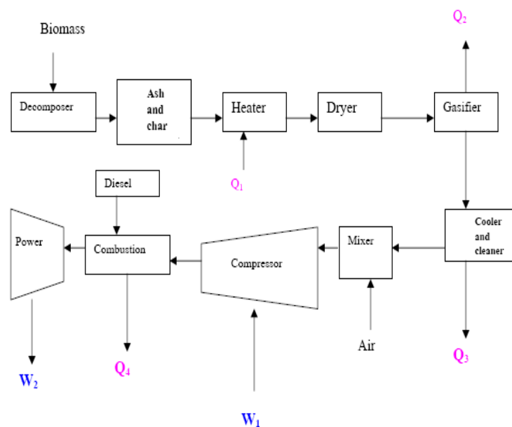
Figure 7. Advanced biomass power with diesel engine (Omer, 2006).
