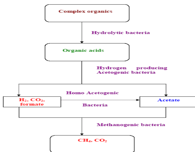
Figure 3. Biogas production process (Omer, 2003).
