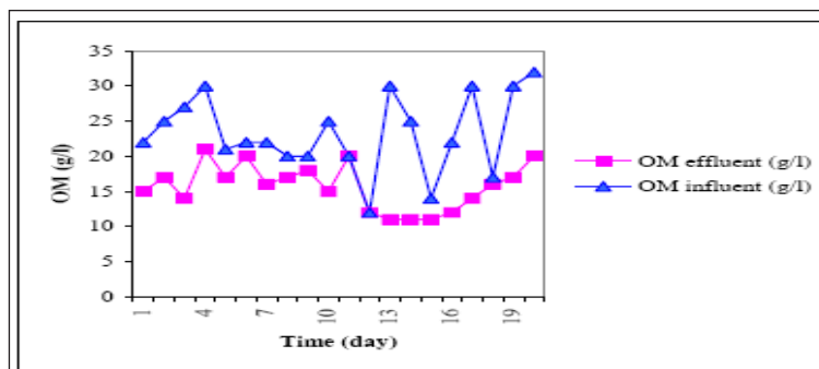
Figure 5. Organic matters before and after treatment in digester (Omer, 2006).
