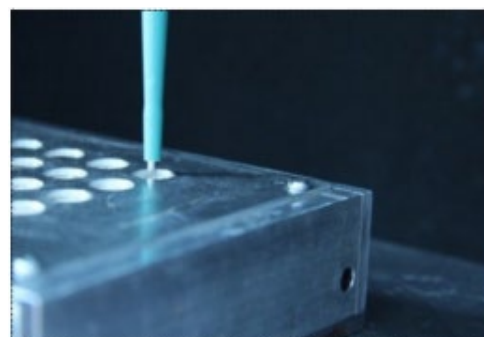
Fig. 5 Perforated plate in the material testing machine
