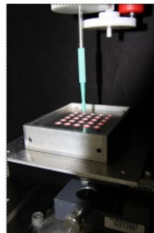
Fig. 4. 2mm biopsy punch in the material testing machine
