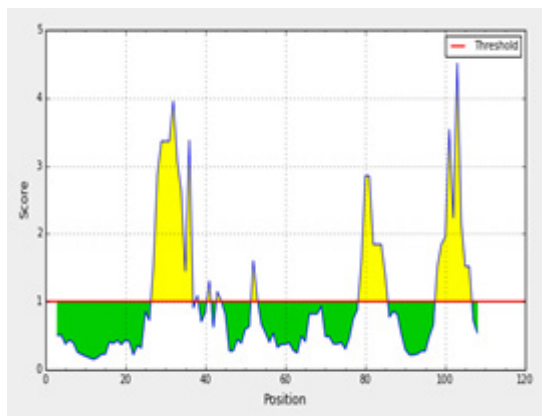
Fig. 5- Emini Surface Accessibility Prediction plot
