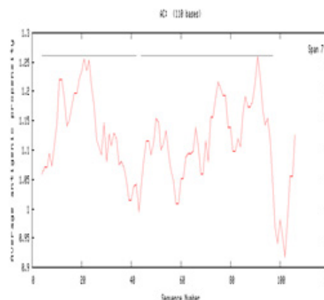
Fig 4a- Kolaskar and Tongaonkar antigenicity plot, the average antigenic propensity for protein 1.1143
