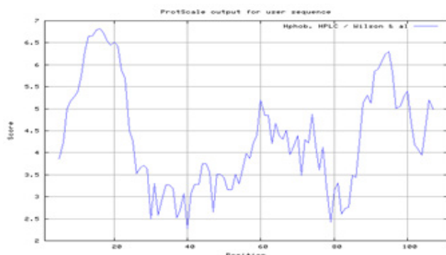
Fig. 10- Hydrophobicity/HPLC plot of Wilson & al (1981)
